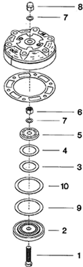
FIGURE 4. LOW PRESSURE CONCENTRIC RING VALVE
